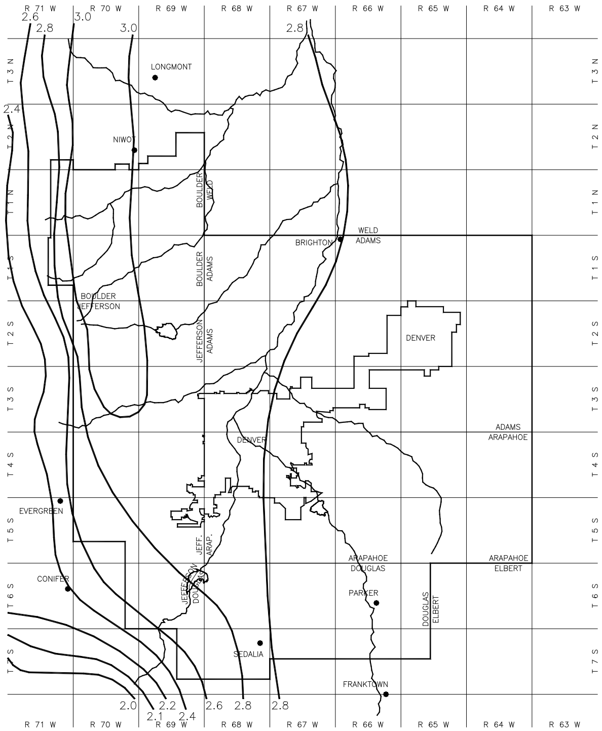
Figure 5-10. Rainfall depth-duration-frequency: 25-year, 6-hour rainfall
