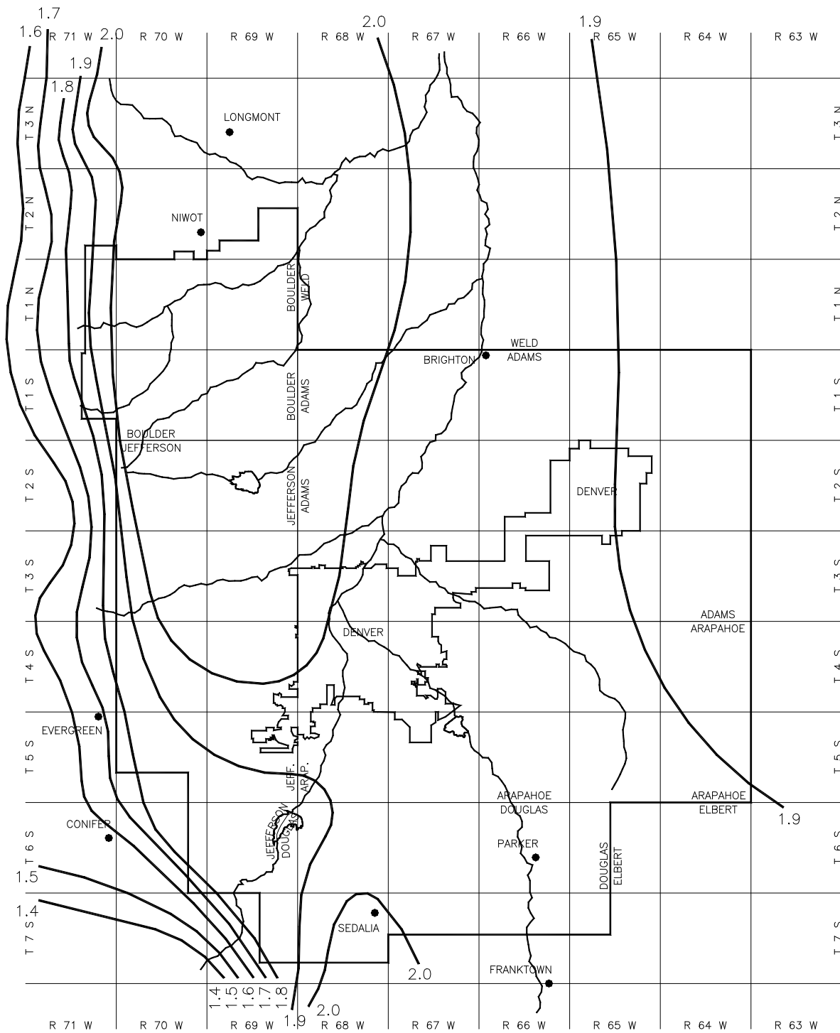
Figure 5-8. Rainfall depth-duration-frequency: 5-year, 6-hour rainfall
