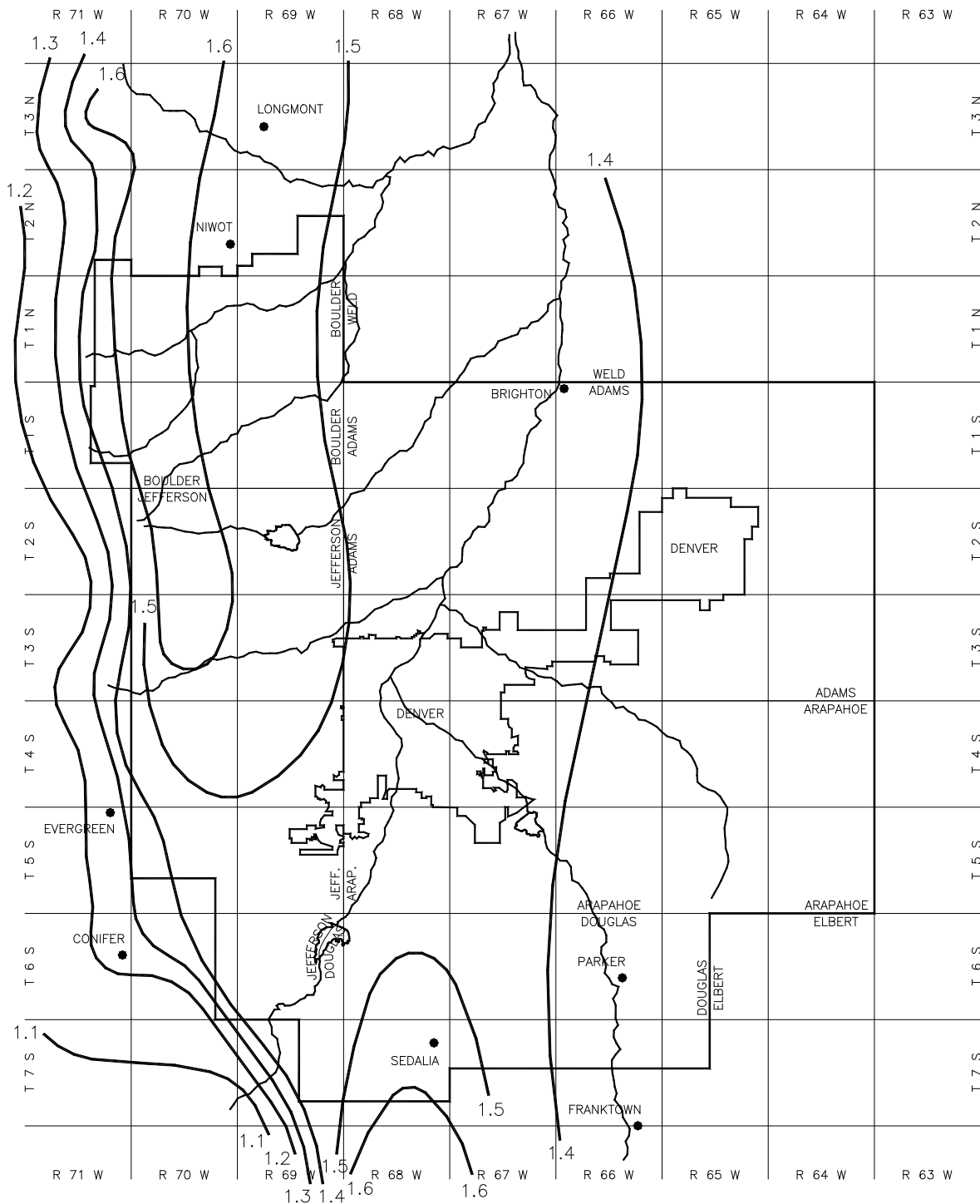
Figure 5-7. Rainfall depth-duration-frequency: 2-year, 6-hour rainfall
