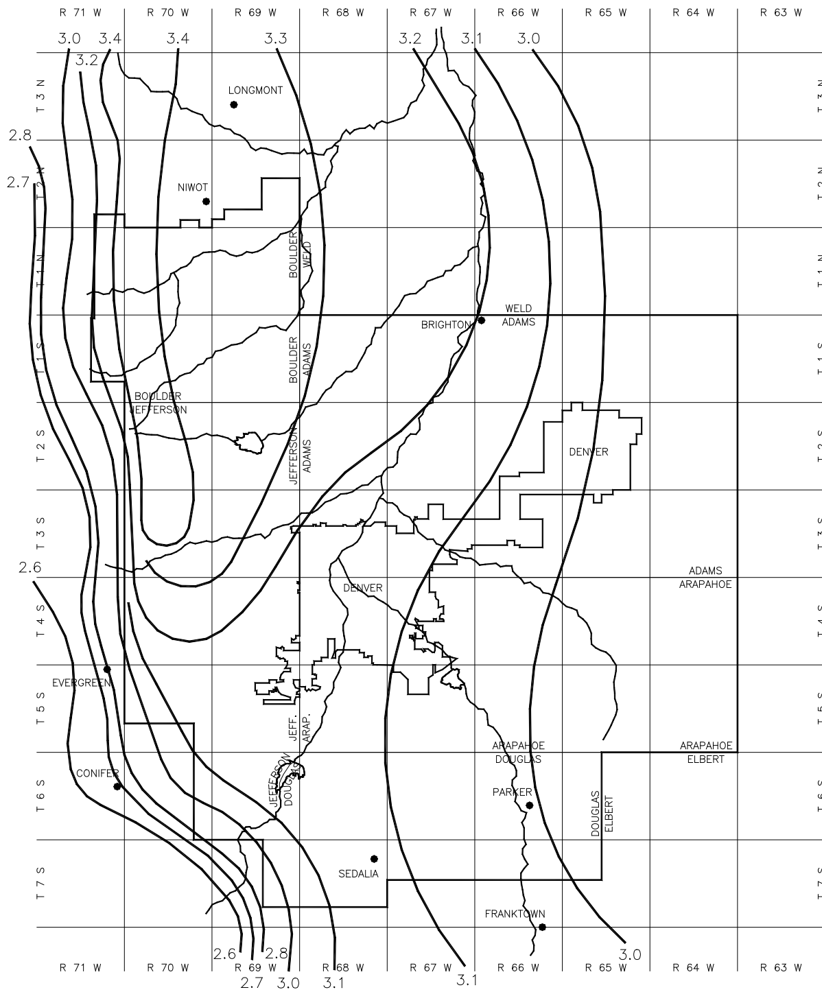
Figure 5-11. Rainfall depth-duration-frequency: 50-year, 6-hour rainfall
