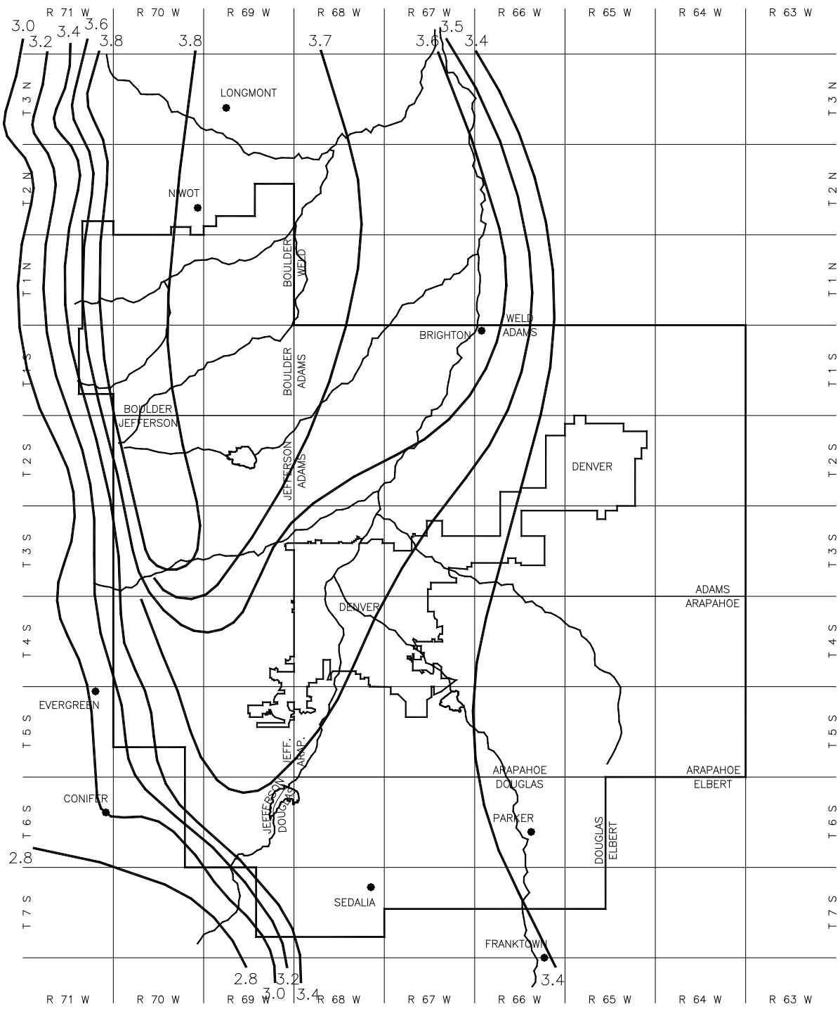
Figure 5-12. Rainfall depth-duration-frequency: 100-year, 6-hour rainfall
