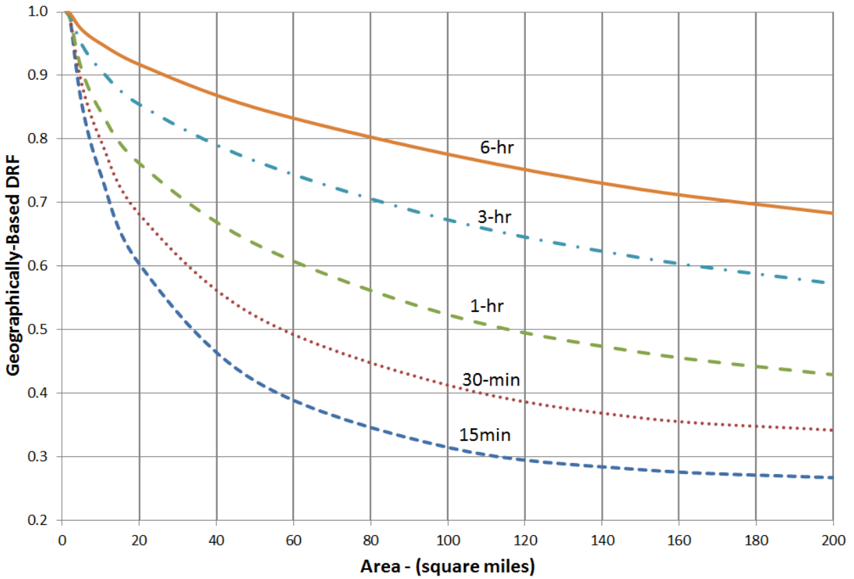
Figure 5-14. Depth reduction factor (DRF) curves for minor storm events (2-, 5-, and 10-year events)
