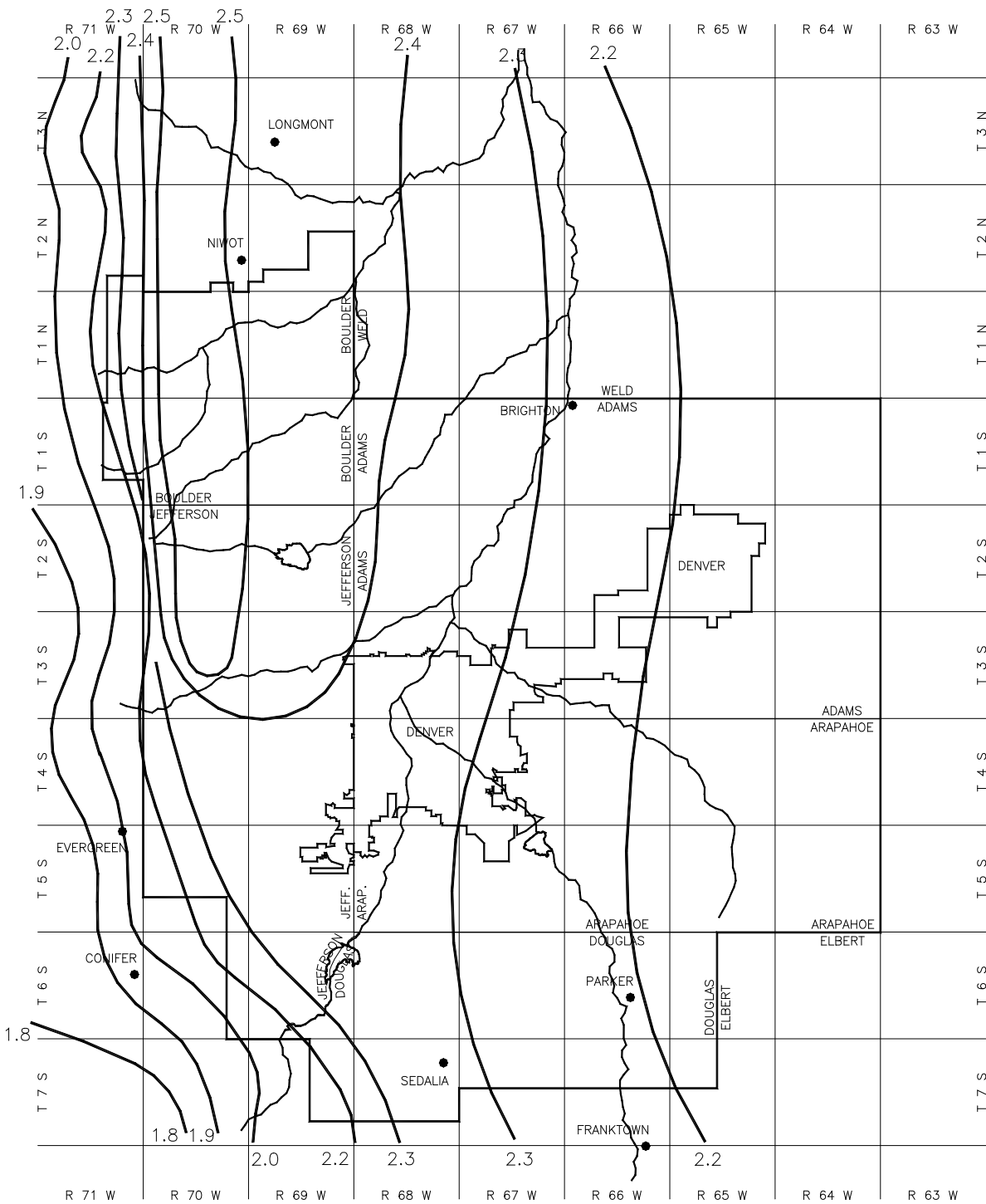
Figure 5-9. Rainfall depth-duration-frequency: 10-year, 6-hour rainfall
