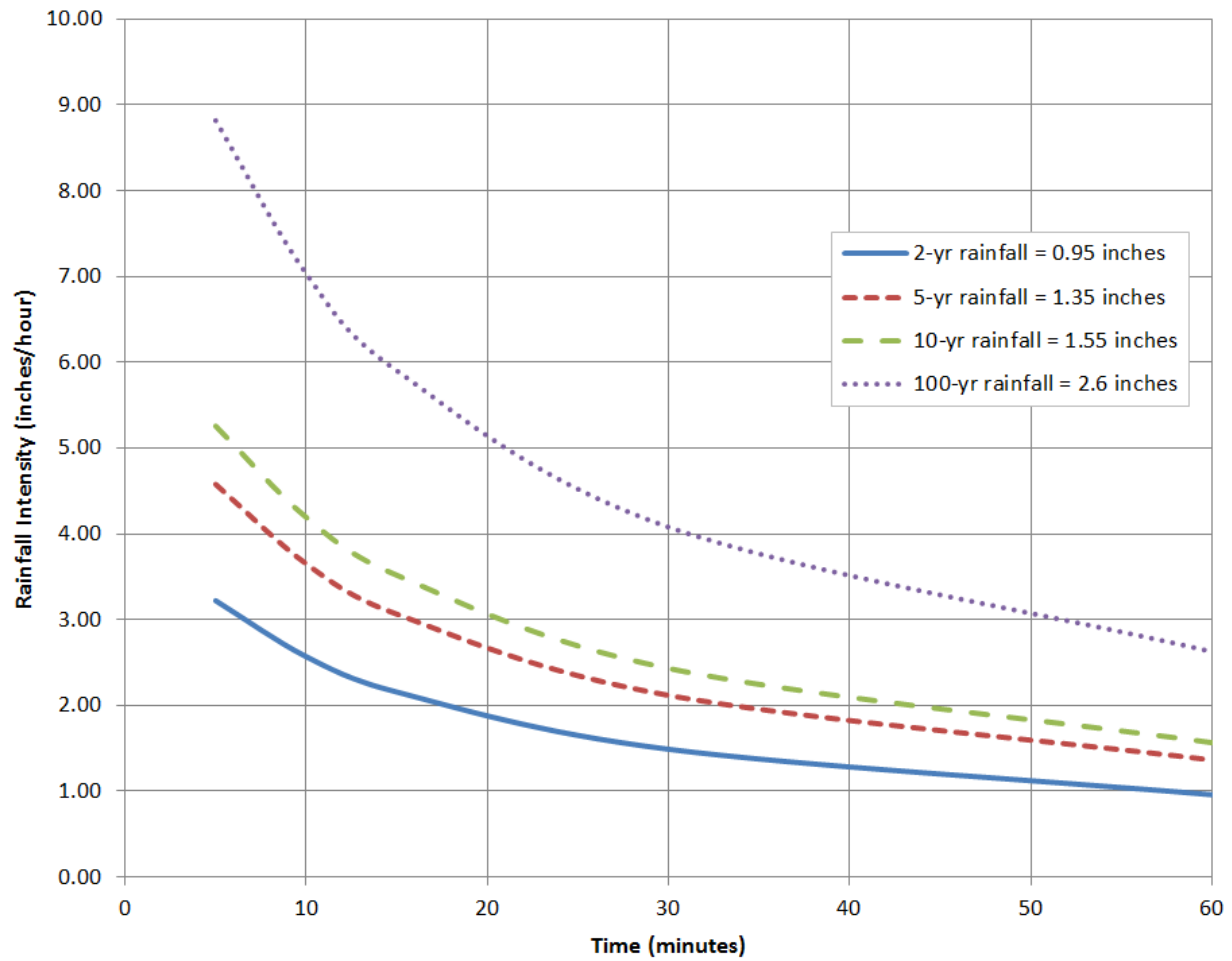
Figure 5-15. Example rainfall intensity-duration curves
