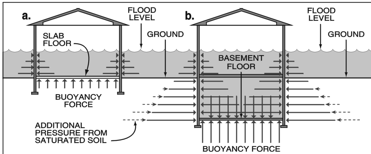
Figure 4-5. Hydrostatic pressure with wet floodproofing (allowing flood waters to enter building)
