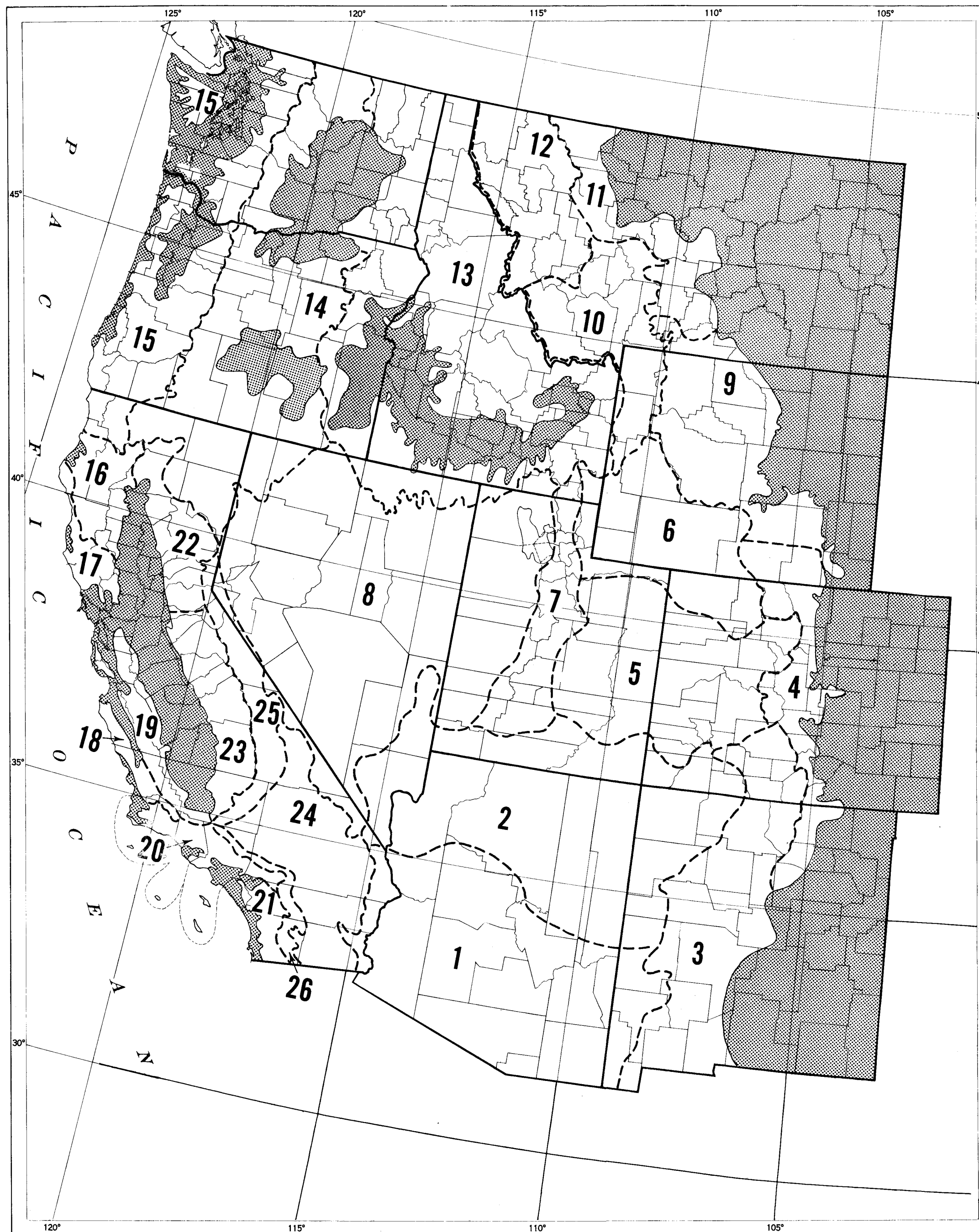
Figure 8. Regions used to develop statistical parameters for interstation interpolation of 2-yr 24-hr precipitation values.
