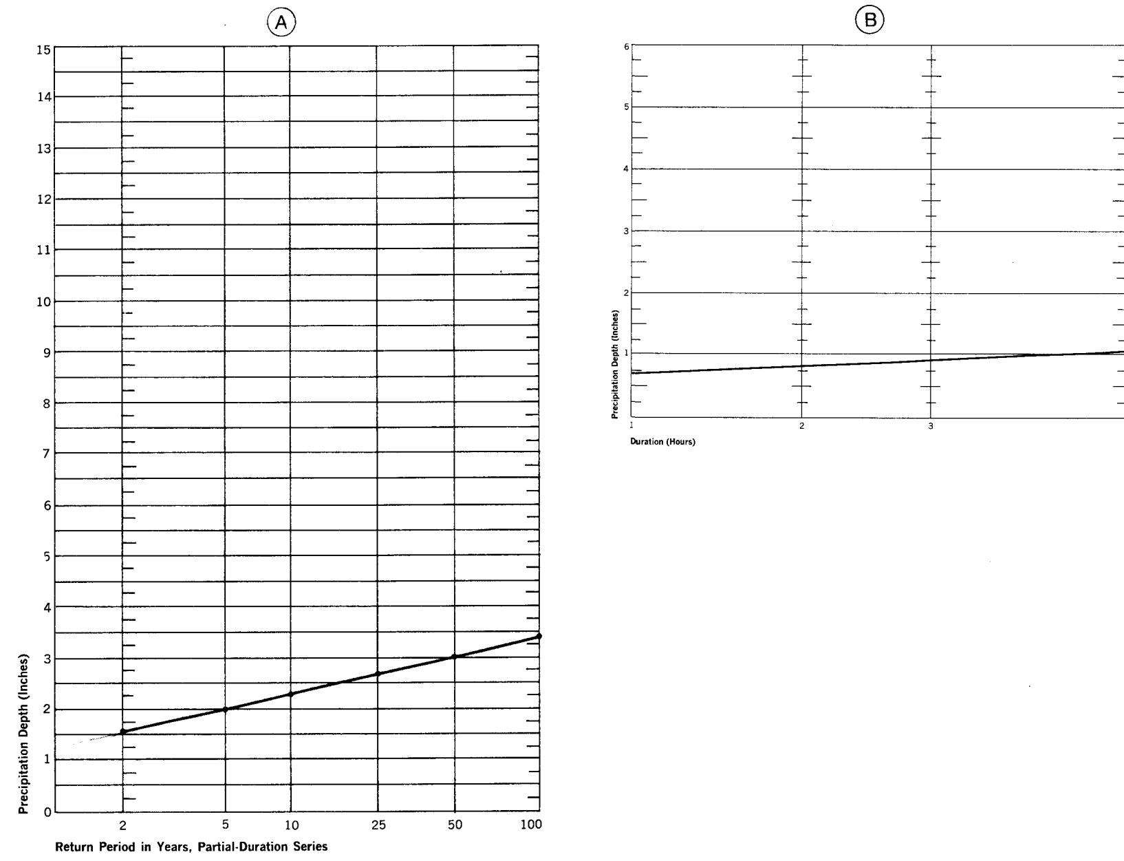
Figure 18. Illustration of use of precipitation-frequency diagrams using values from precipitation-frequency maps and relations at 106°00' W., 39°00' N.
