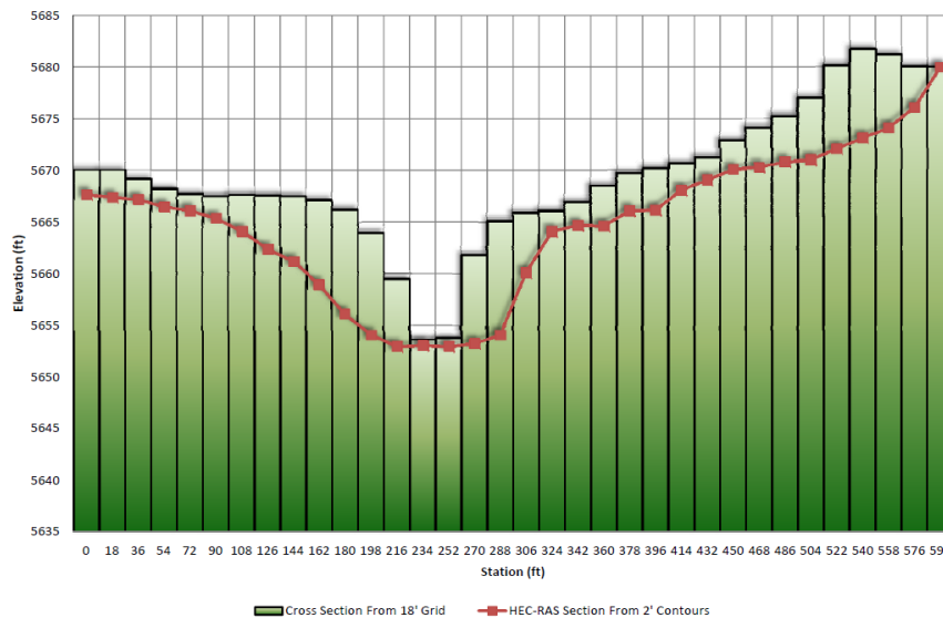
Figure 3 – Comparison of Cross section from HEC-RAS vs. from FLO-2D 18' Grid
