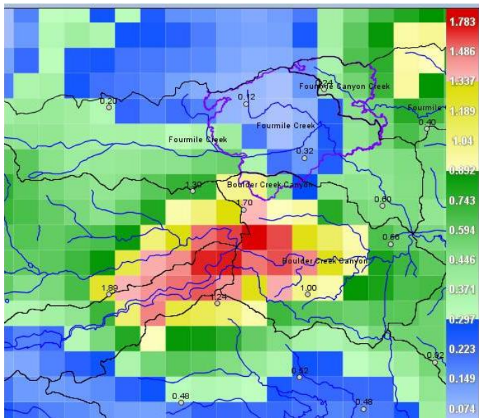
Radar-rainfall estimates between 5-8 pm, July 7
