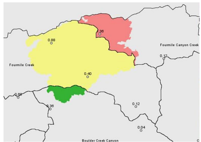
Colors represent Radar estimates of average rainfall over the FMBA by watershed thru 9PM. The yellow area (Fourmile Creek drainage) reflects an average rainfall of 0.7". The red area (Fourmile Canyon Creek drainage) reflects an average of 1.2". The green area (Bummers Gulch drainage) averaged 0.5". The numbers are ALERT rain gage totals. Sunshine measured the highest amount of 1.36".
