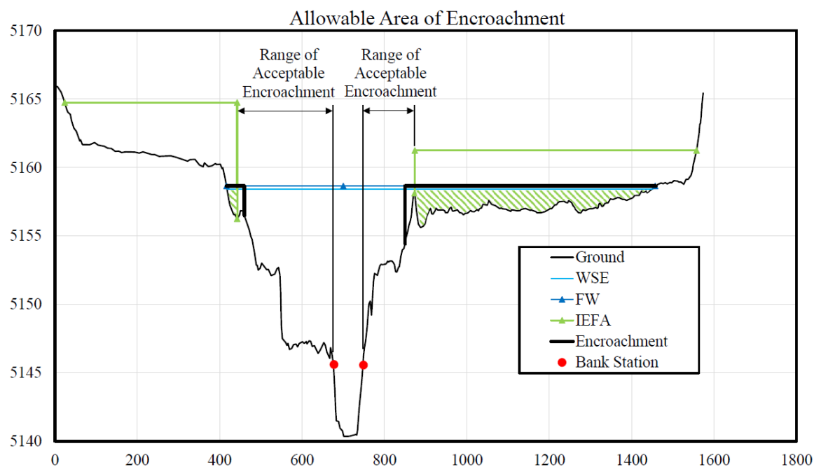
Figure 2-4. Allowable Area of Encroachment
