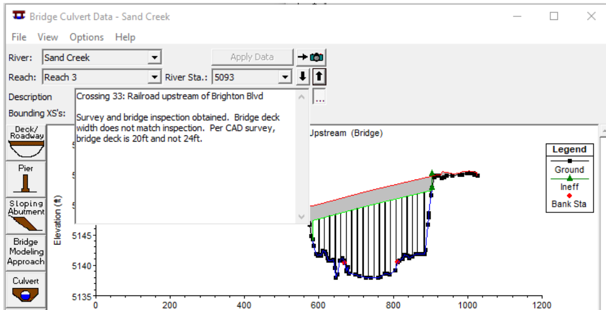
Figure 2-2. Using the HEC-RAS Description Boxes
